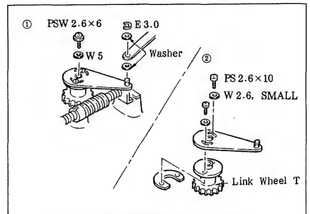
Fig. 6-67. Replacement of Link Wheel T
